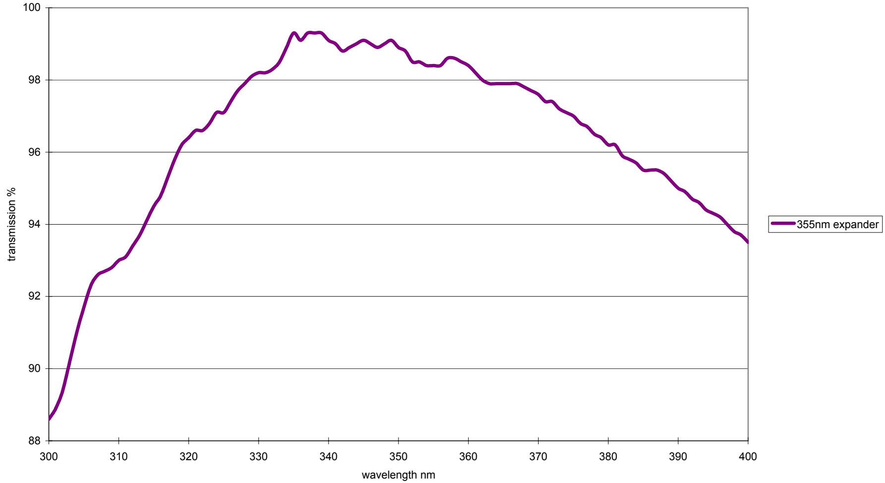
Typical Transmission for Geomatec Brand 355nm Fixed Ratio Expander www.beamexpander.com
