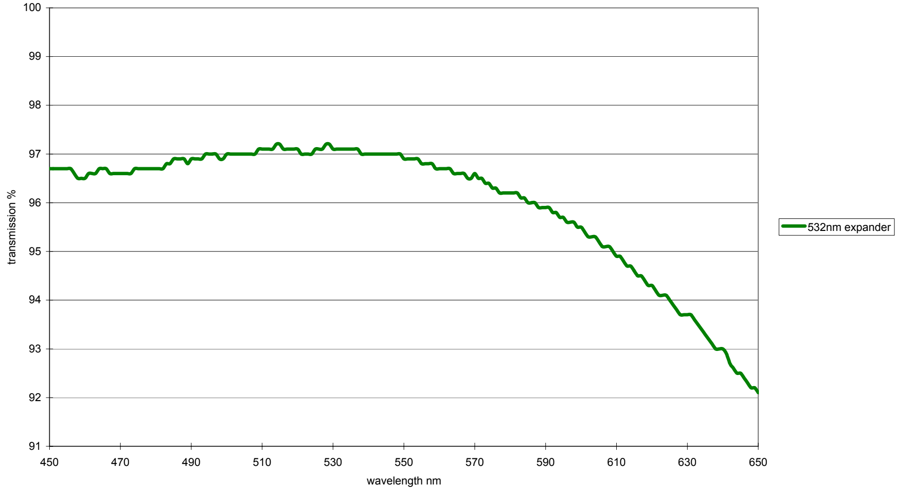
Typical Transmission for Geomatec Brand 532nm Fixed Ratio Expander www.beamexpander.com
