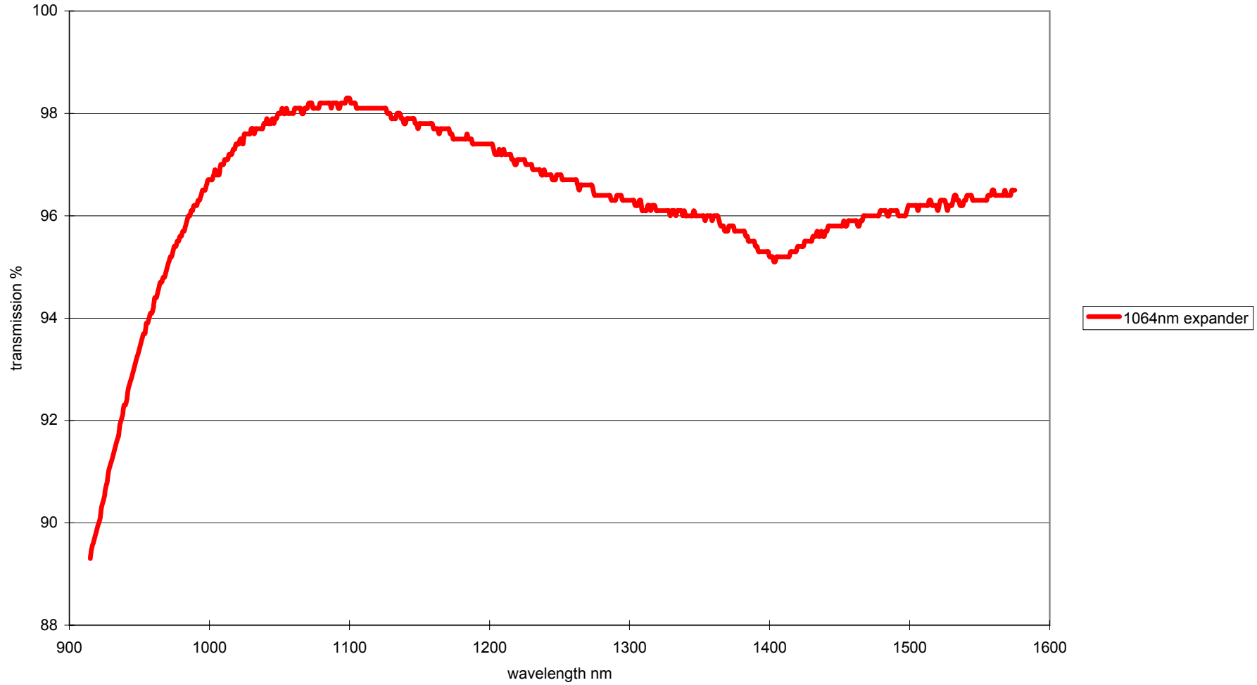
Typical Transmission for Geomatec Brand 1064nm Fixed Ratio Expander www.beamexpander.com
